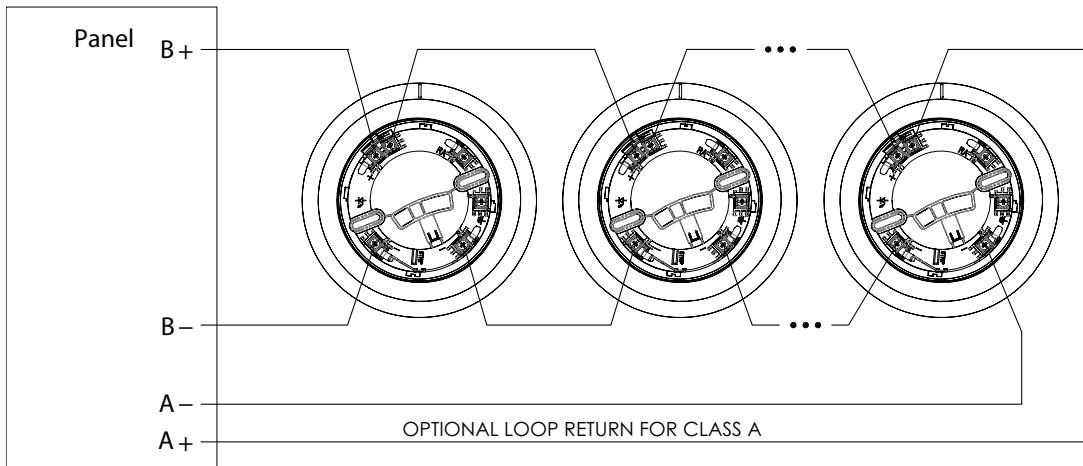
FIGURE 3: LOOP WIRING
