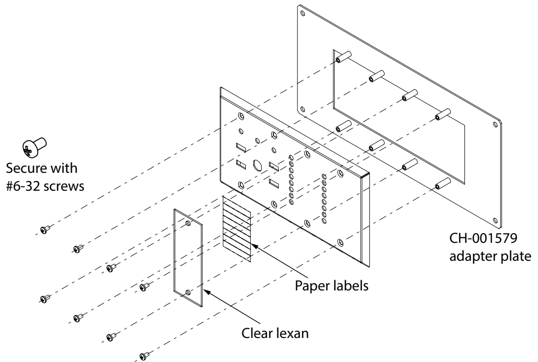
Figure 1 Secure MR-2306-AT to CH-001579
