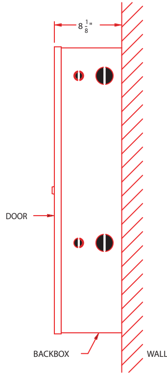
SURFACE (SIDE VIEW)
