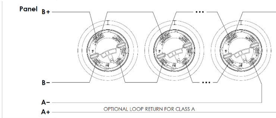
FIGURE 3: LOOP WIRING
