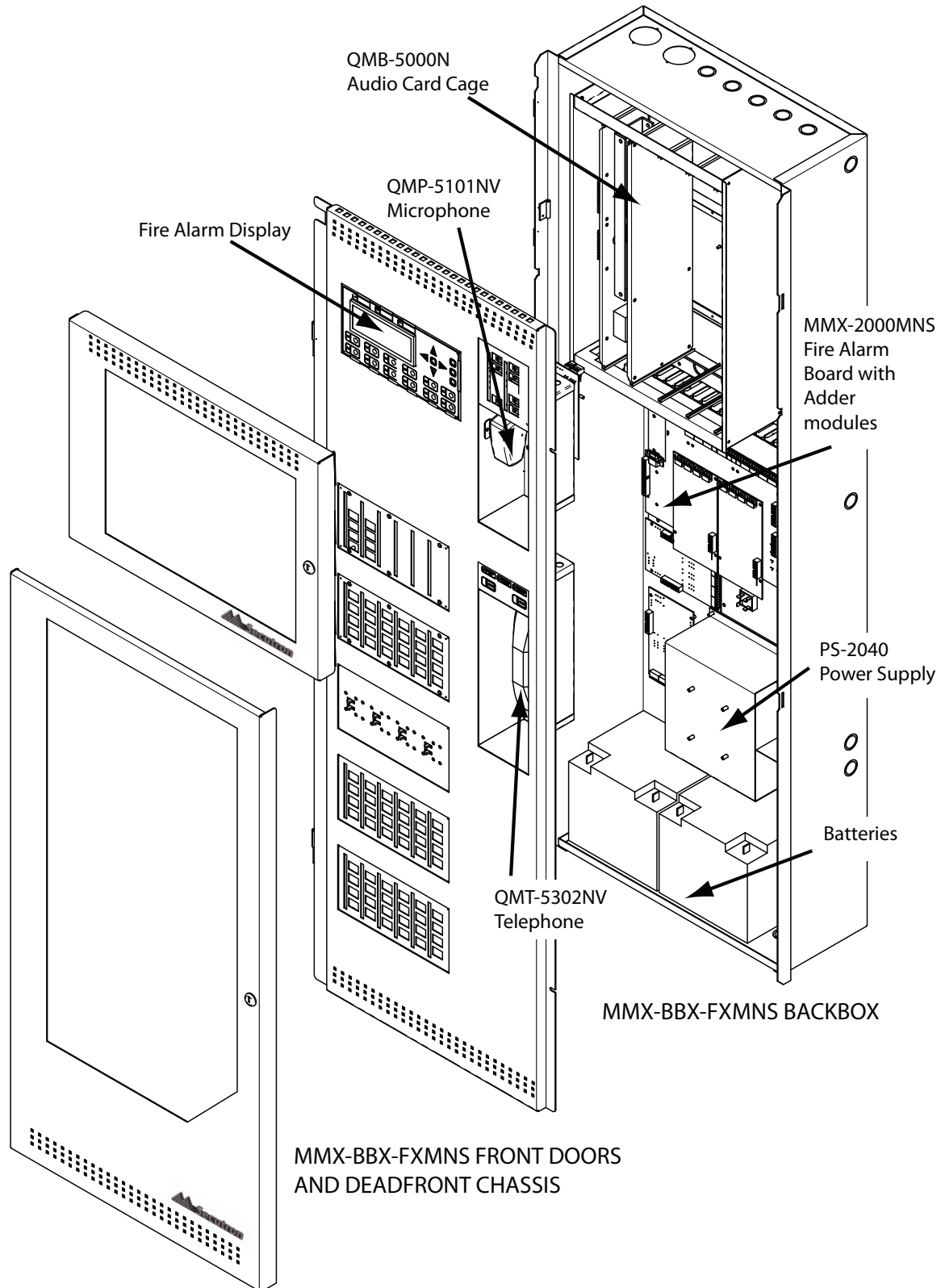
Figure 2: Expanded View of the MMX-BBX-FXMNSG Enclosure
