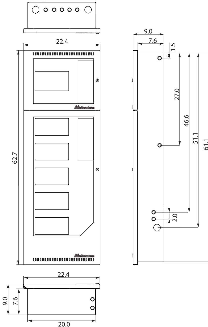
Figure 1: MMX-BBX-FXMNSG Enclosure with Dimensions (inches)
