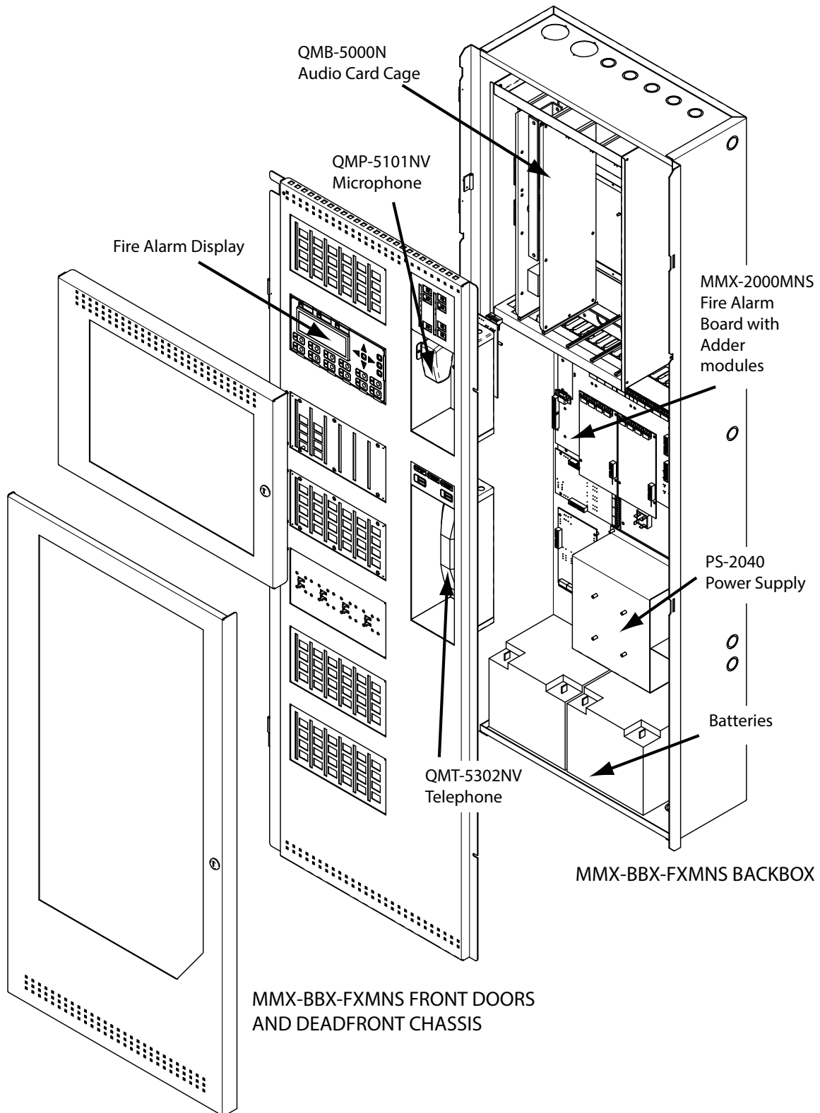
Figure 2: Expanded View of the MMX-BBX-FXMNS Enclosure
