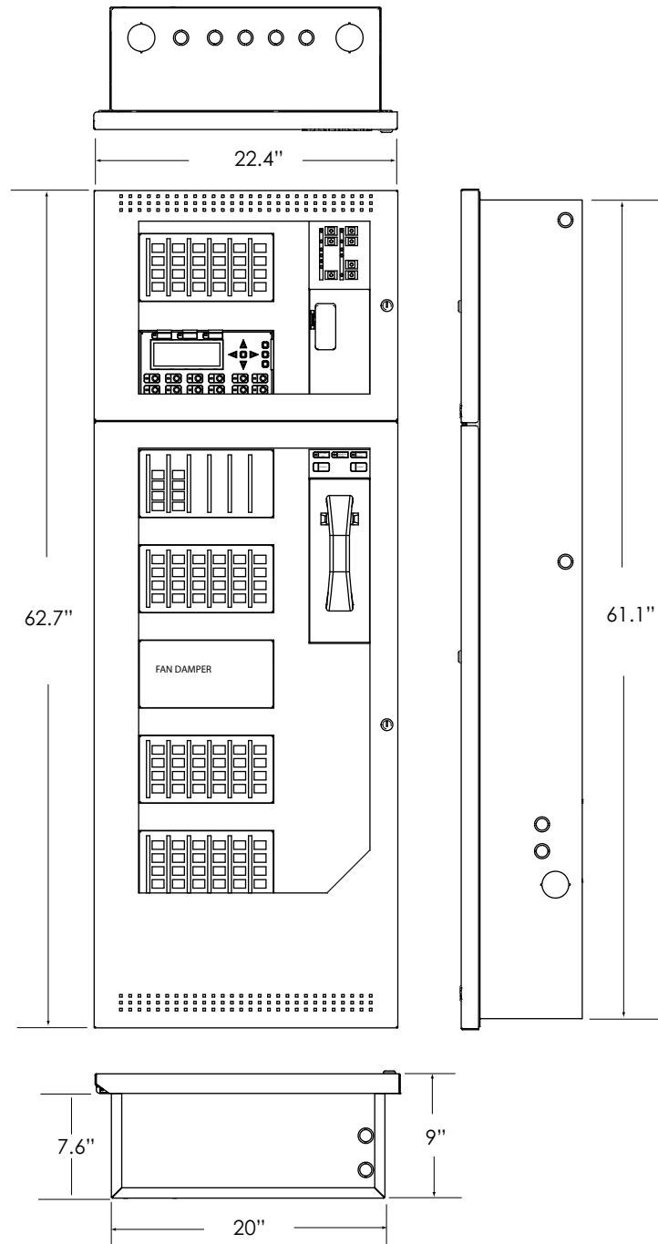
Figure 1: MMX-BBX-FXMNS Enclosure with Dimensions
